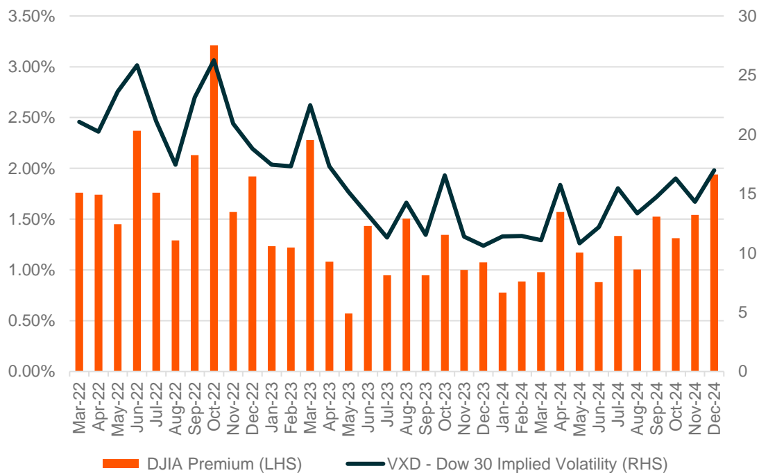
DJIA Premium % vs. VXD (1-Month DJX Implied Volatility)
