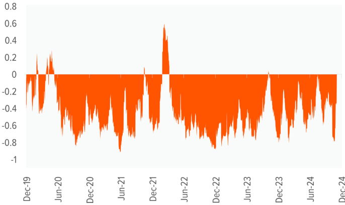
GOLD AND DOLLAR CORRELATION - 30 DAYS ROLLING
