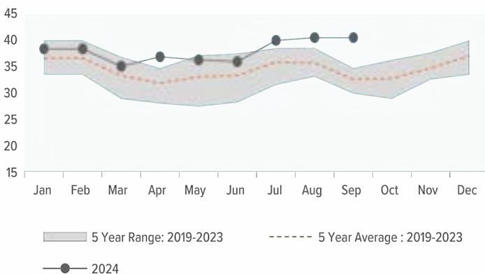
CHINA NUCLEAR POWER GENERATION (BILLION KWH)
